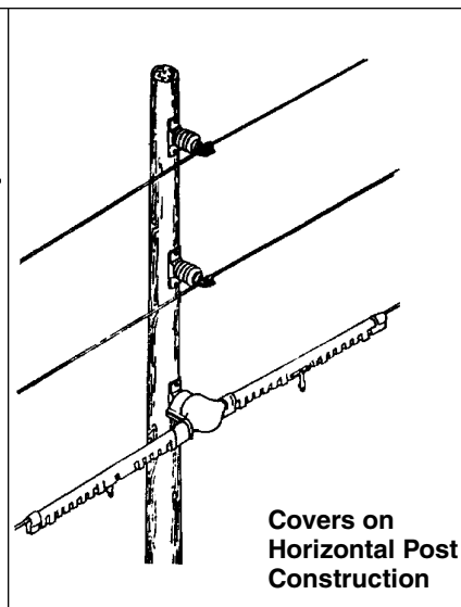
P4060185 and P4060186 without Grip-All Adapter for rubber-glove application
